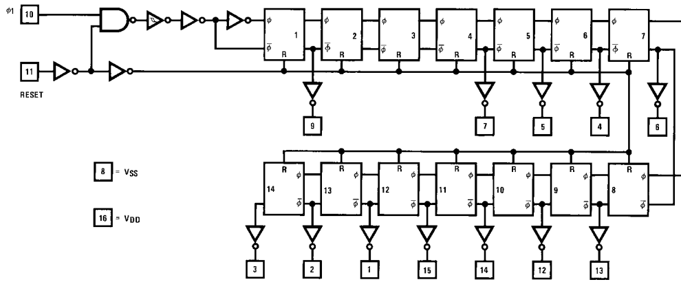
CD4020BC
